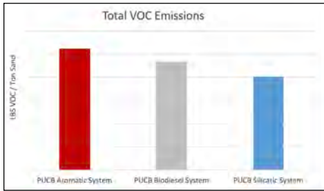
Graph 3 - Example of total VOC emissions in comparison (OCMA & PCS) *systems tested at 1.3% total binder level and 55/45 Pt1to Pt2 ratio
